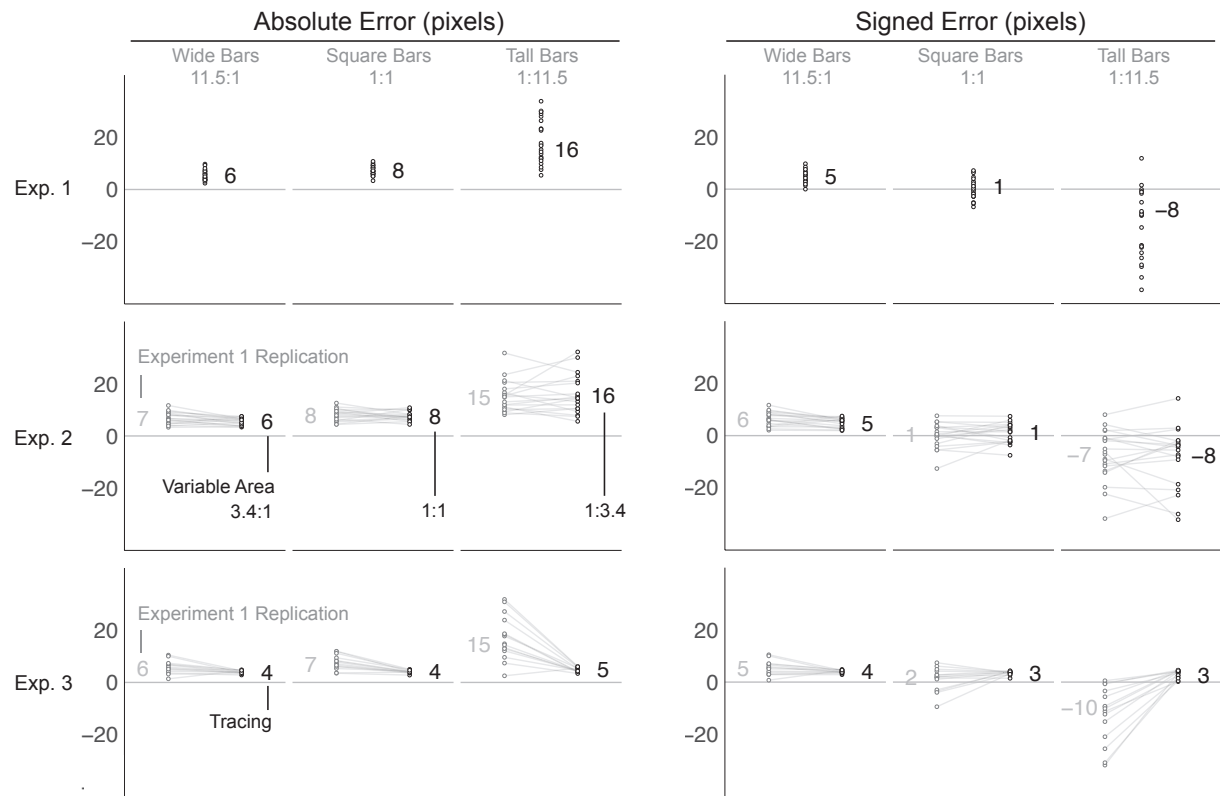
Fig. 6. Absolute error (pixels) and signed error (pixels) for Experiment 1, 2, and 3. Each dot indicates the mean error for a single participant in each corresponding experiment, and annotated numbers are the mean error in pixels for all participants. All light gray dots are for Experiment 1 or its replications in Experiments 2 and 3. All black dots are the manipulated conditions (Experiment 2: variable area condition; Experiment 3: tracing condition). The aspect ratios of the bar marks were wide (11.5:1), square (1:1), or tall (1:11.5) for all conditions but the variable area condition in Experiment 2.
