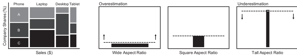
Fig. 1. The Mekko chart at left uses height to encode relative market share, similar to a bar chart. But the present results suggest that the aspect ratio of each mark may bias this height judgment. When asked to reproduce the vertical position of a single bar mark in a bar chart, bars with wide aspect ratios were overestimated, bars with tall ratios were underestimated, and bars with square ratios showed no systematic bias. This pattern of bias appeared within memory, suggesting that value comparisons that occur across time and space (e.g., bars in separate graphs) would most likely be distorted.
