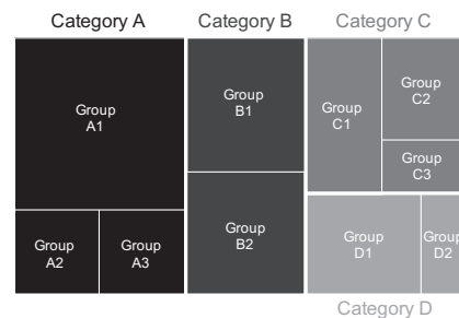
Fig. 4. A simple treemap. Each category differs in color; within each category are nested groups.
